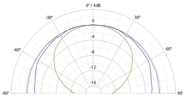
Polar pattern (1m) Purple = 200Hz / Blue = 1kHz / Yellow = 5kHz
